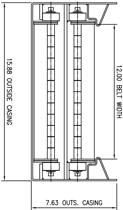
VIEW THRU CASING @ LOAD SECTION SCALE: (DOUBLE)
